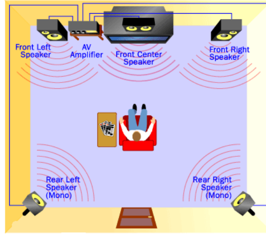
Dolby Pro-Logic Installation 2x front stereo speakers 2x rear mono speakers 1x center speaker
